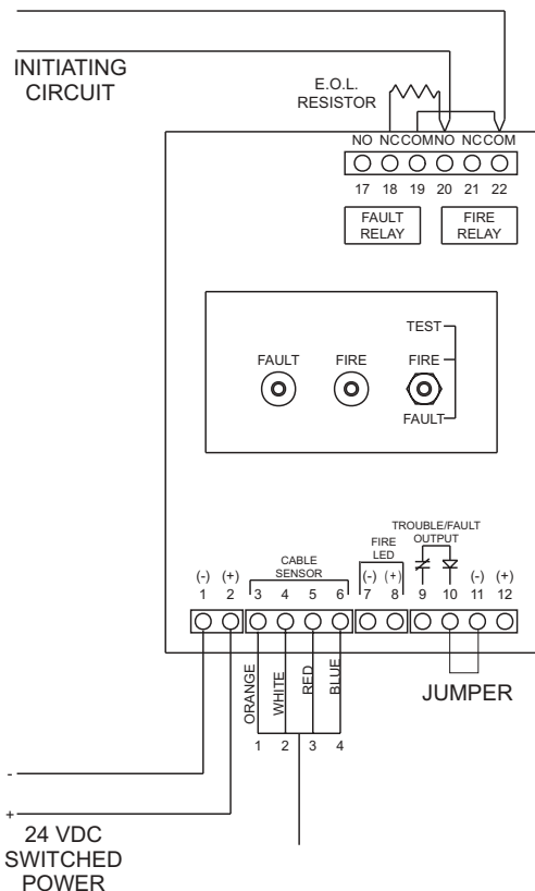
Figure 5. 4-Wire Module Wiring Diagram
