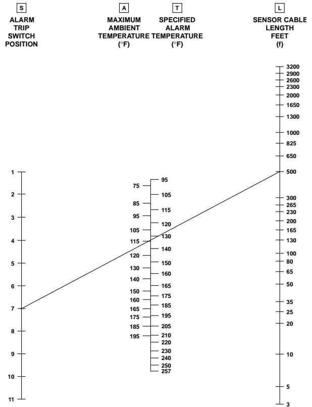
Figure 2. Example for Type "T" Cable
