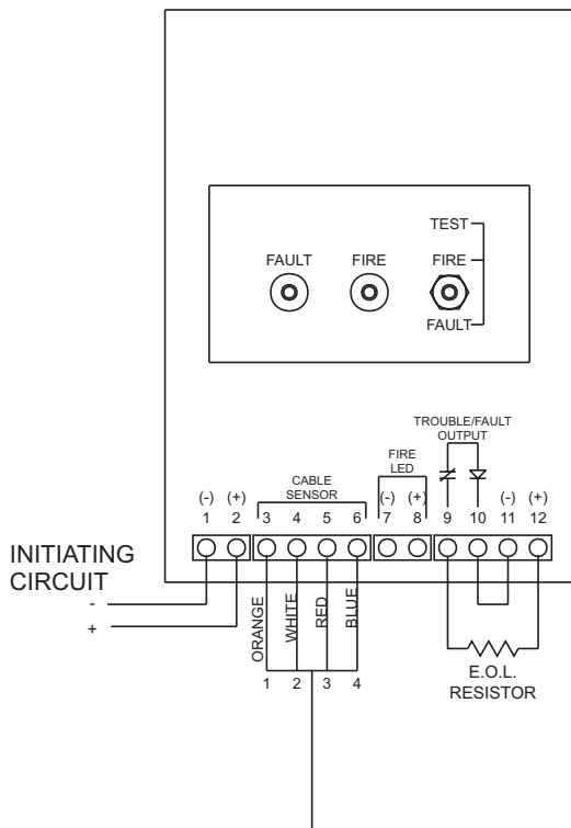
Figure 4. 2-Wire Module Wiring Diagram
